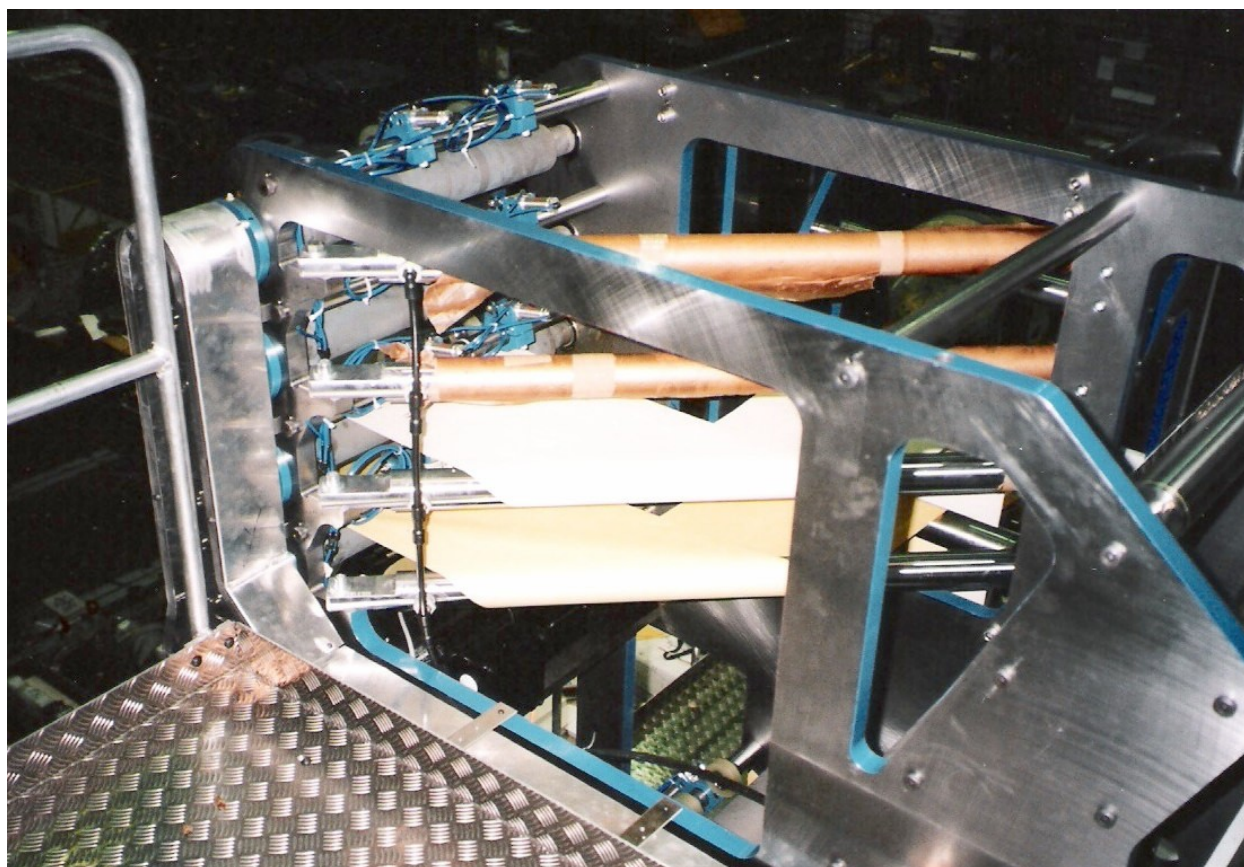
Ribbon Bypass Anglebars mounted above the double former. Four lead capacity.
