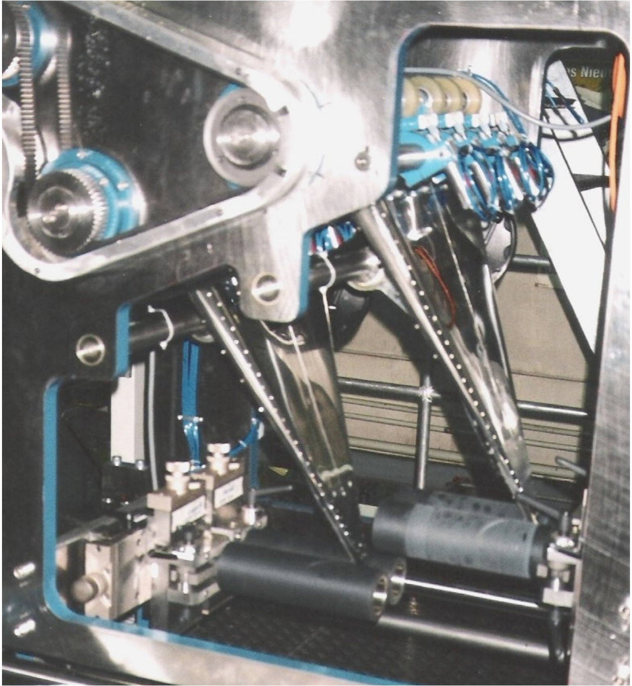
Double Former Section, Independently Driven
